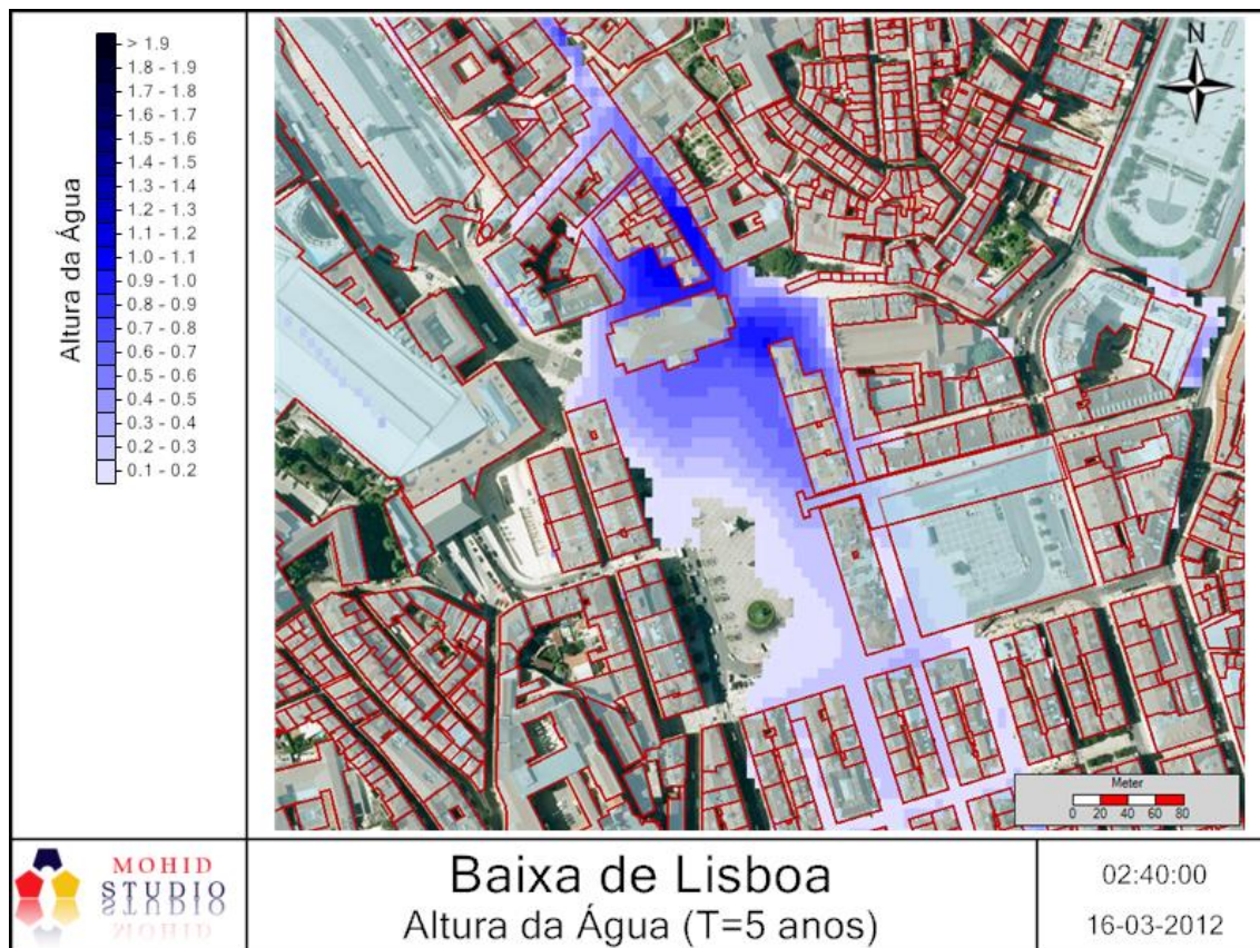
Figure 24: Maximum inundation level for an historic event occurred in 2008
