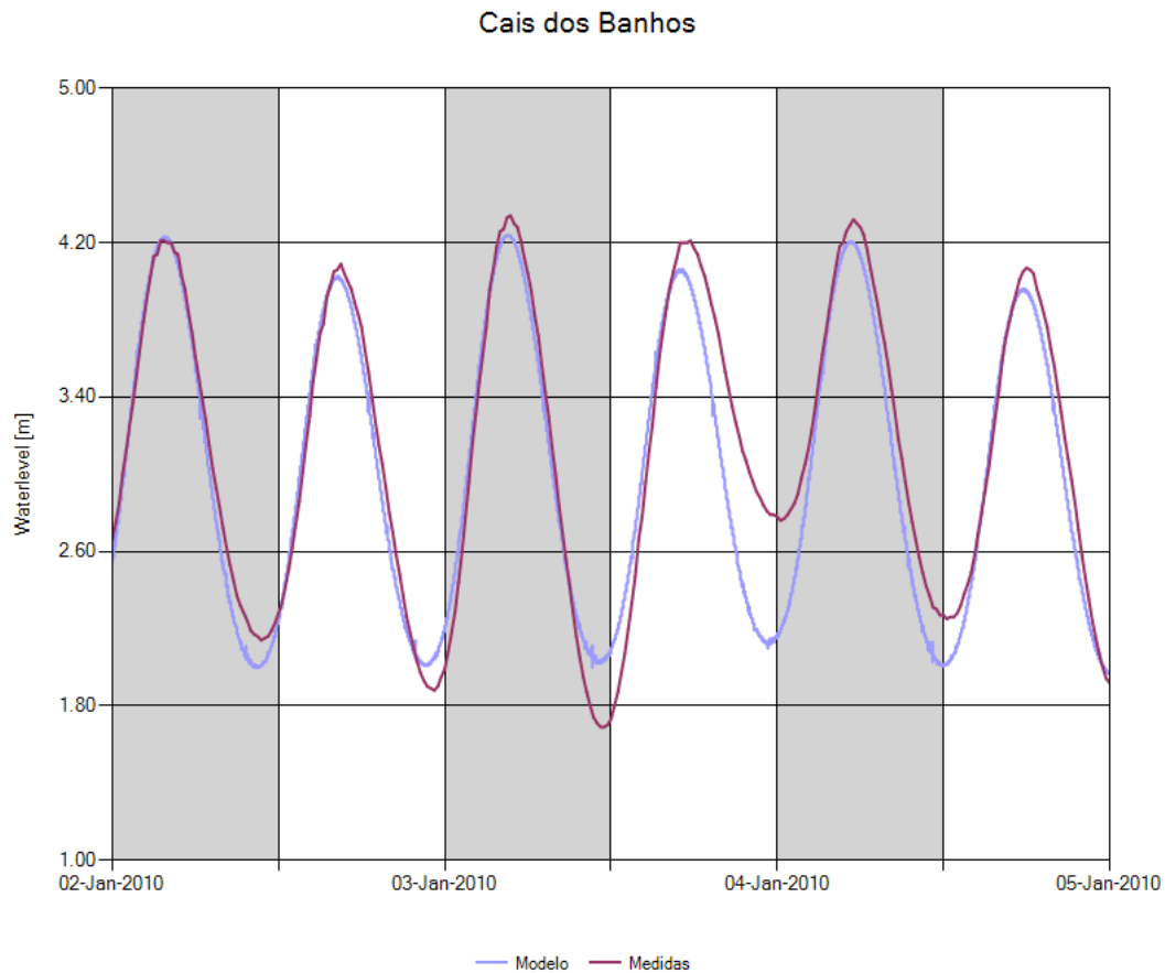
Figure 34: Comparison of modeled and observed water levels (Cais dos Banhos)
