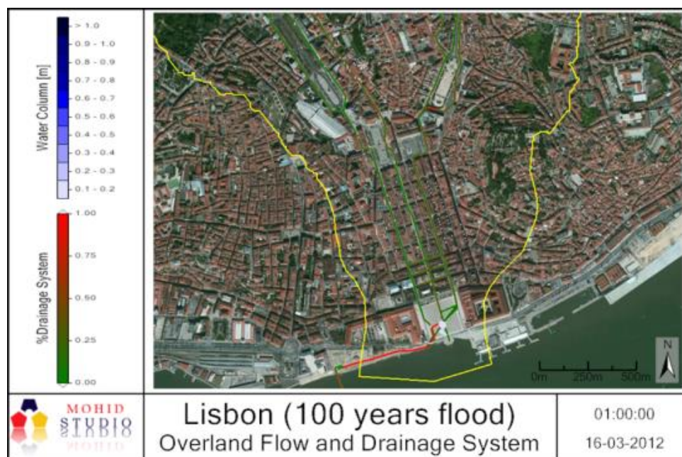
Figure 21: Propagation of a 100 year flood in Lisbon downtown (after 1h)
