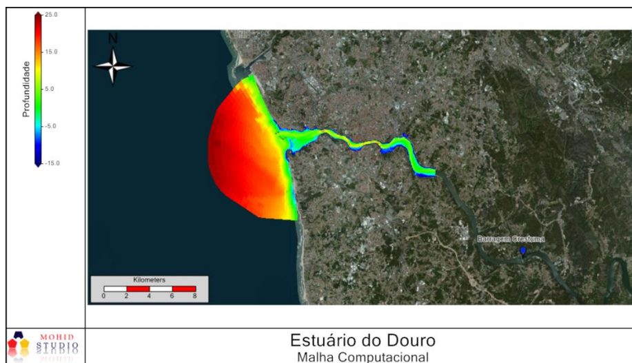
Figure 33: Computational grid used in Oporto
