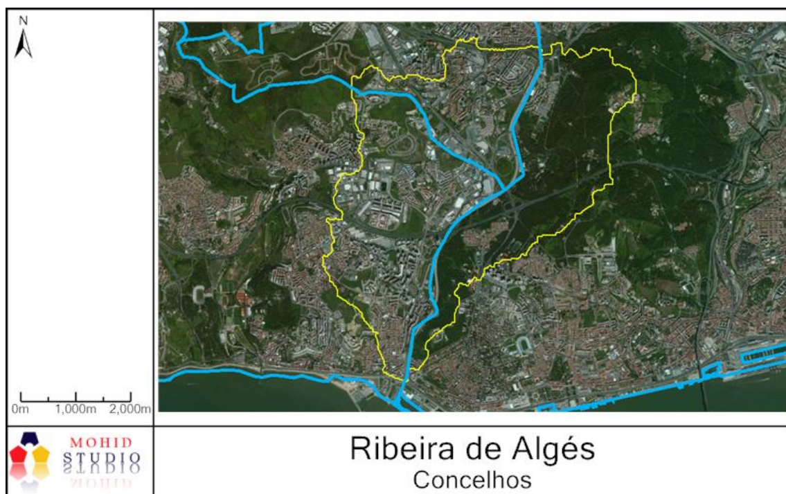
Figure 5: Boundaries of the watershed (yellow) and the intersecting municipalities (blue)
