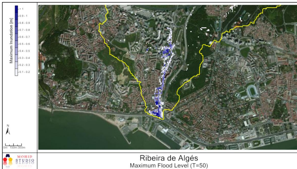
Figure 14: Maximum expected inundation depth (T=50 years)
