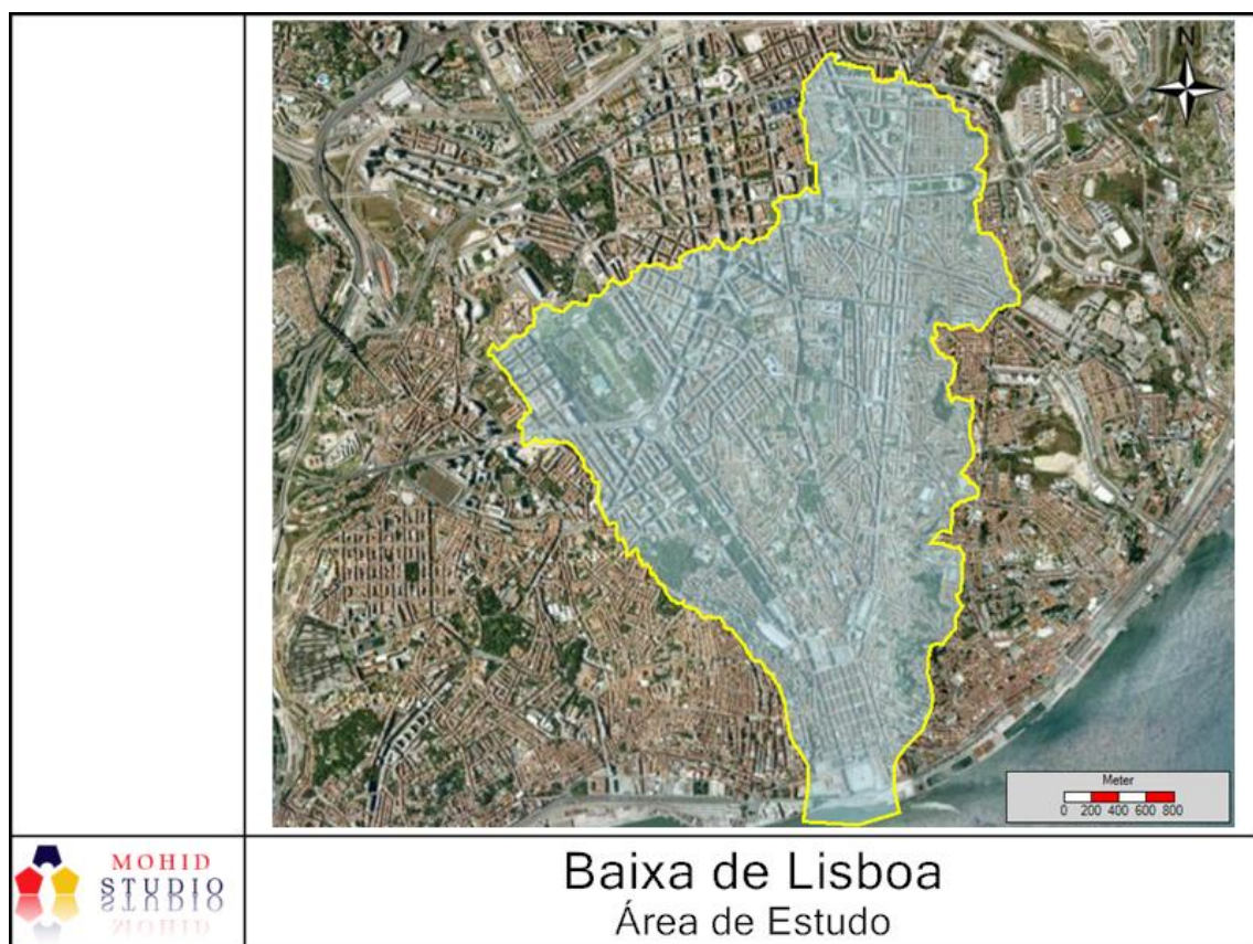
Figure 16: Boundaries of the watershed (yellow)
