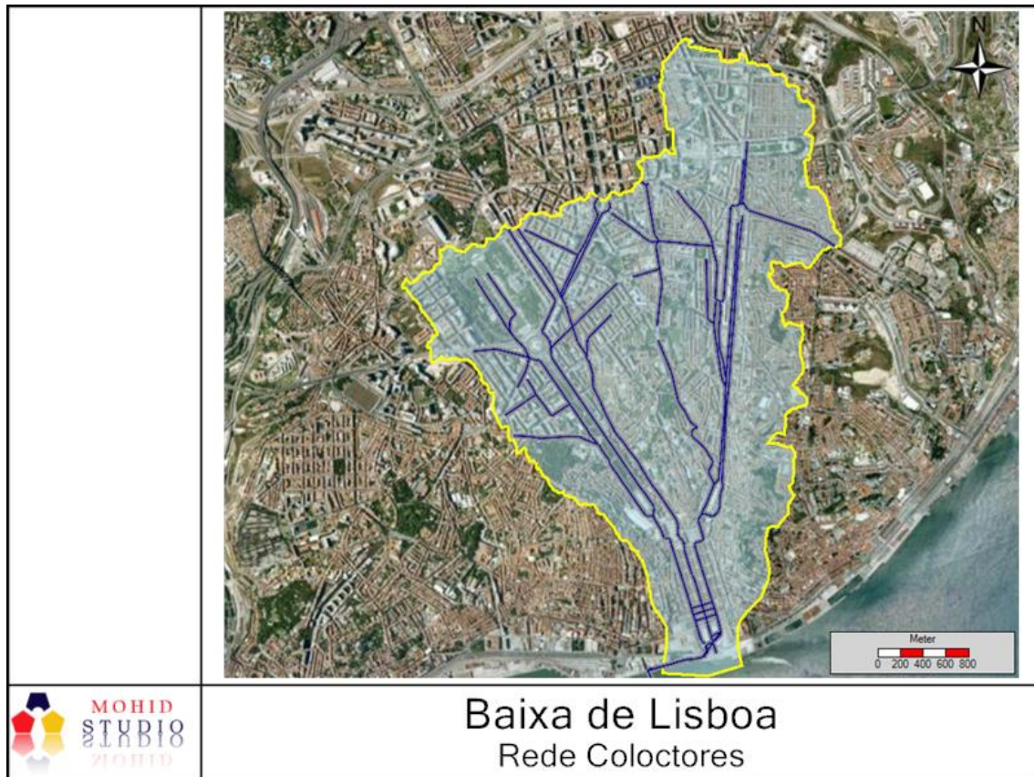
Figure 18: Storm water drainage system simulated by the SWMM model
