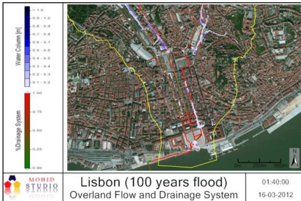
Figure 22: Propagation of a 100 year flood in Lisbon downtown (after 1h 40min)
