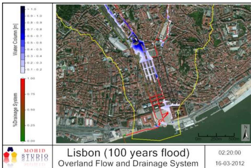
Figure 23: Propagation of a 100 year flood in Lisbon downtown (after 2h 20min)
