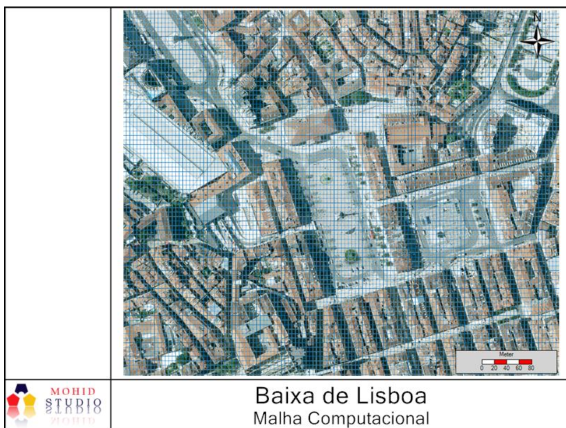
Figure 17: Zoom of the computational grid used for MOHID Land (Praça de Rossio)
