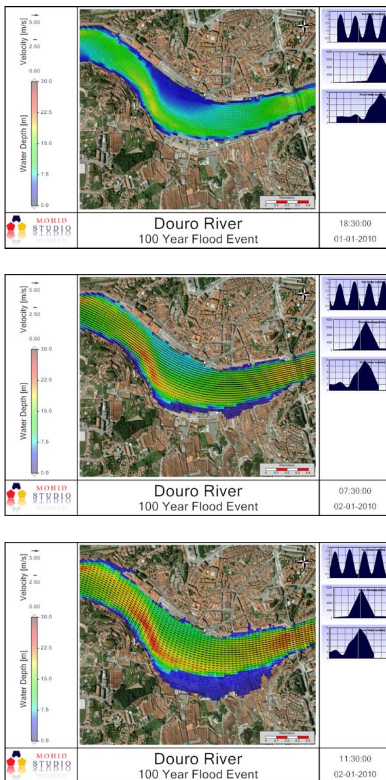
Figure 35: Different instants during a 100 year event (Douro River)
