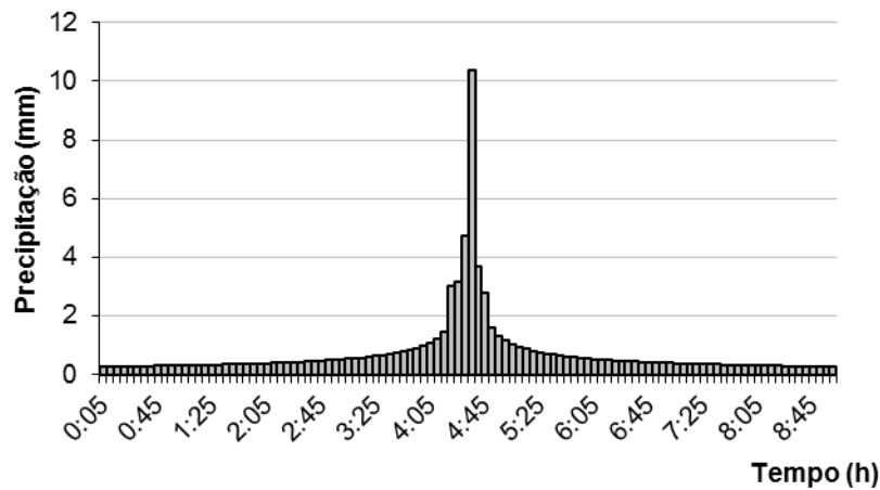
Figure 12: Design event of a 100 years flood
